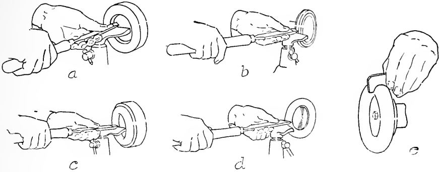
FIG. 326. TURNING A RING—SECOND METHOD.
